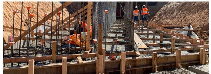
Carpenters and iron workers constructing the bridge support system footing for the new Van Buren Boulevard bridge.
