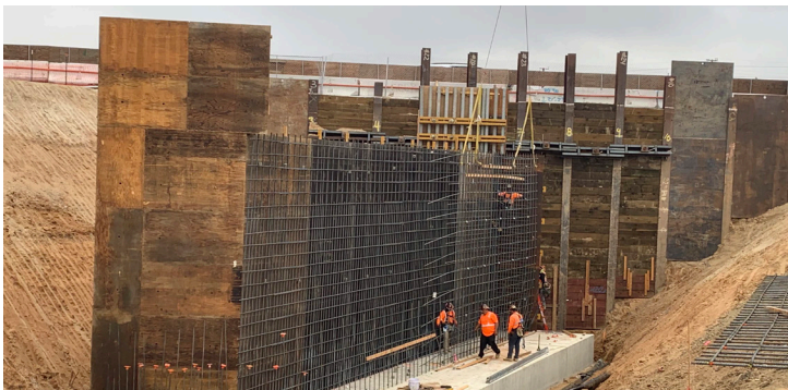
Iron workers placing rebar on the Van Buren Blvd. bridge support abutment in preparation for the upcoming concrete placement.
