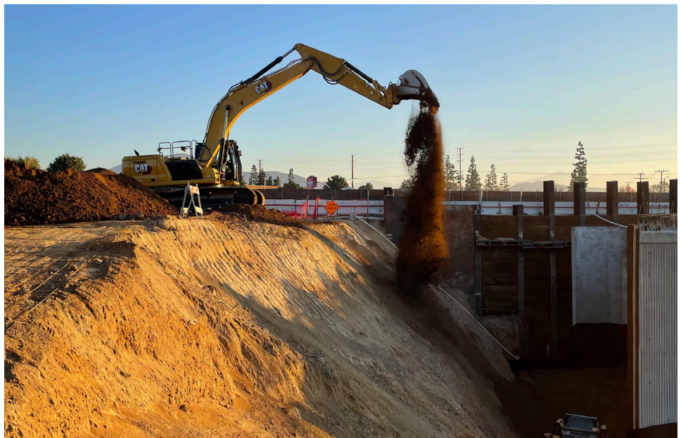
Looking east, crews are backfilling the north end of the Van Buren Boulevard bridge support system.
