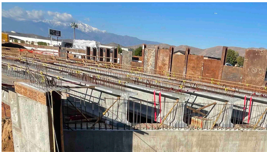
A north facing view of the Van Buren Boulevard bridge retaining wall and support system. Once these are finished, the next step is to construct the bridge deck.
